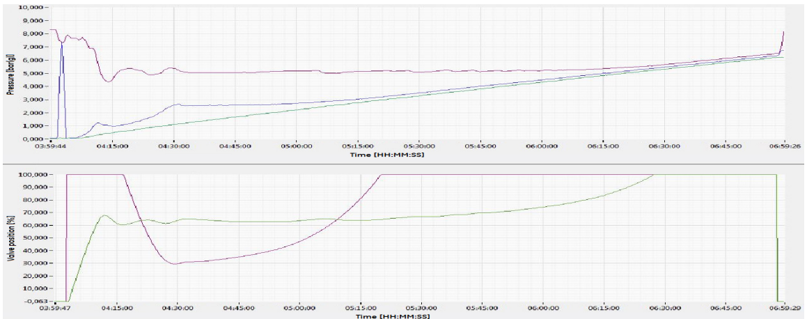
Fig. 4. Pressure at the adsorption dryer (red), pressure at the second stage control valve (blue) and pressure in the spherical air storage units (green) over time
