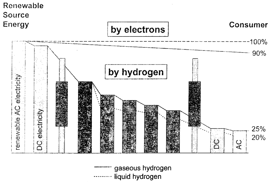
Fig. 9. Electricity Transport
