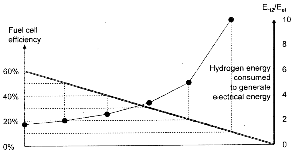
Fig. 13. Fuel Cell Efficiency and Hydrogen Consumption
